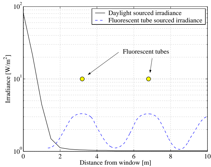
Fig. 2. Comparison of indoor irradiance source measurements, based on Fig. 3.28 in [22].
