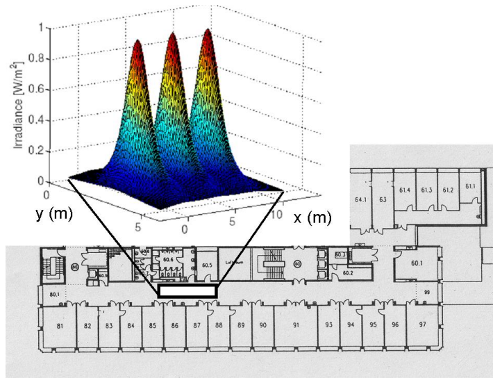
Fig. 5. Example of a simulated radiant intensity distribution as 3D plot for the scenario
