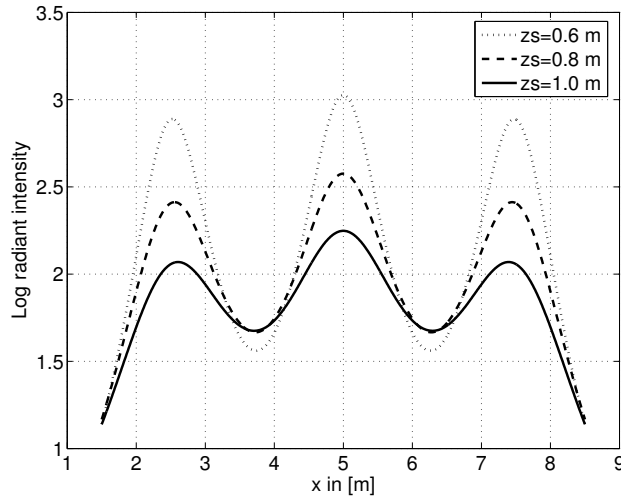
Fig. 4. Simulation of a movement along x under three point sources in 2.5 m spacing at different ceiling distances z_S of \underline{S} ( y_S = y_0 ).
