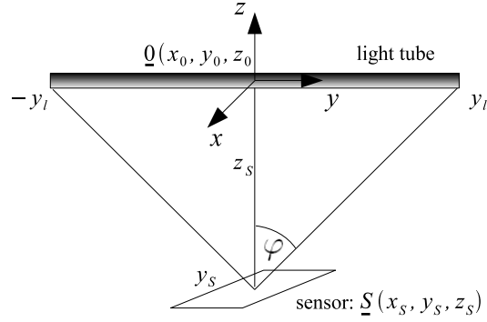
Fig. 3. Schematic for the light emitter model
