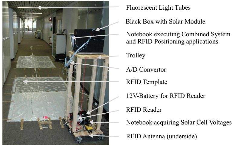
Fig. 8. Measurement trolley and prepared test track.
