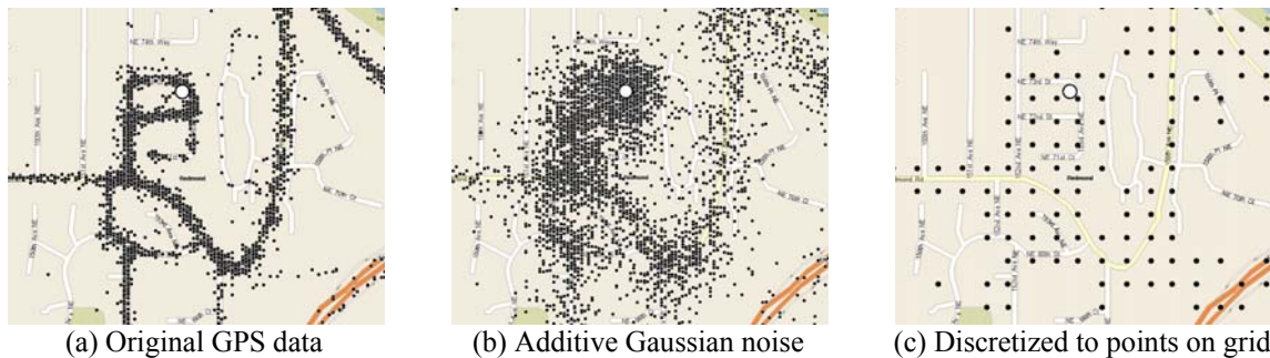
Figure 1: Obfuscation can enhance location privacy, e.g. by adding noise or discretizing to a grid. From [29].
