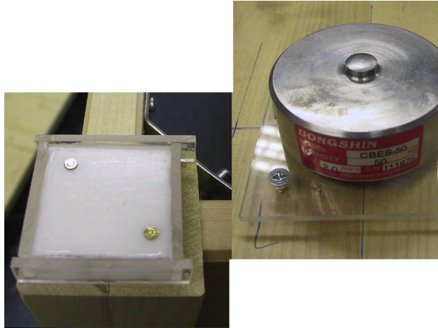
Figure 5. resting point and load cell mounted under the table top of a dinning table.
